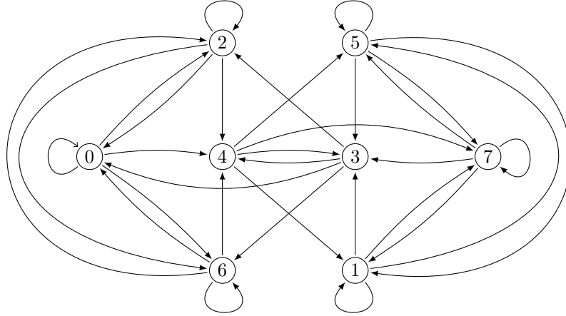
Figure 2.6: Directed graph D
