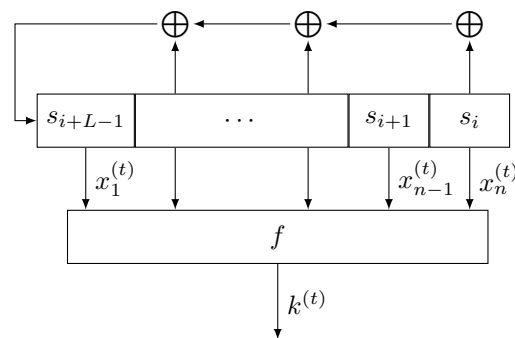
FIGURE 1 – Filtrage de LFSR
